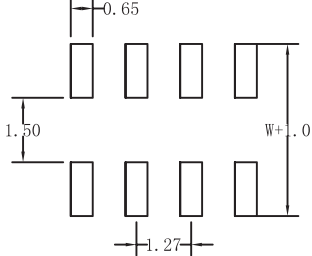
Recommended P. C. Board Hole Layout
